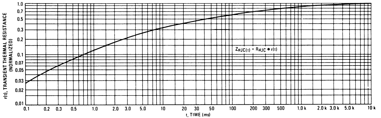
FIGURE 5 – THERMAL RESPONSE
