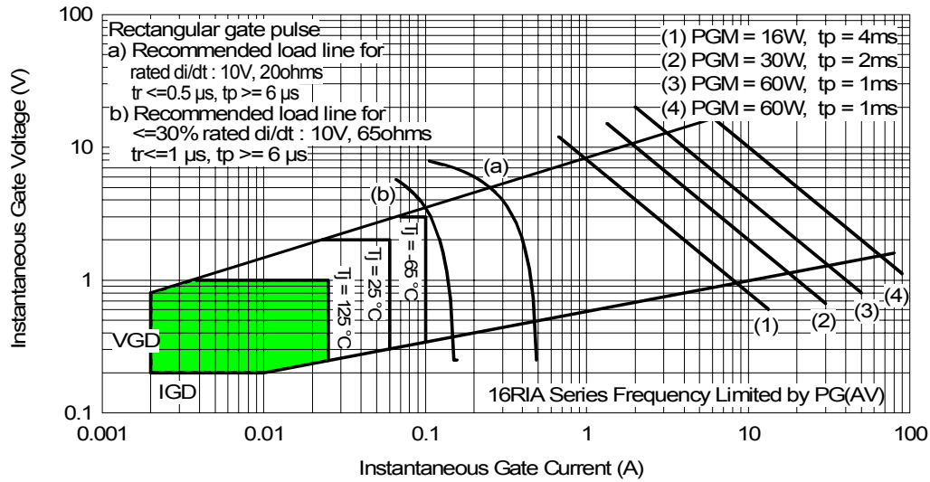
Fig. 16 - Gate Characteristics
