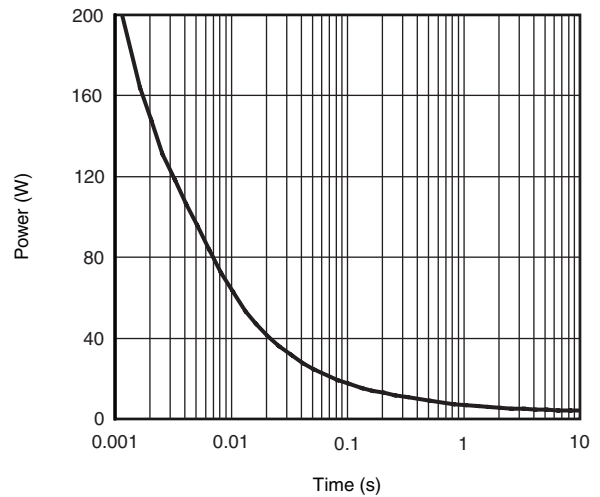
Junction-to-Ambient
