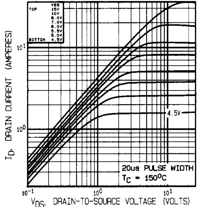
Fig 2. Typical Output Characteristics
