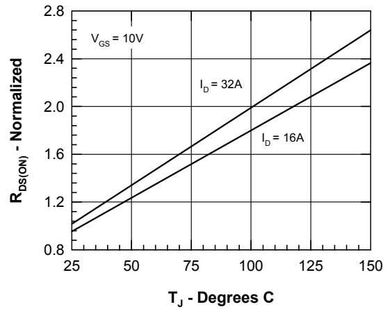
Figure 4. R_{DS(on)} normalized to 15A/25°C vs. T_J
