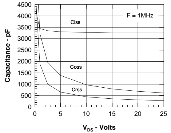
Figure 8. Capacitance Curves
