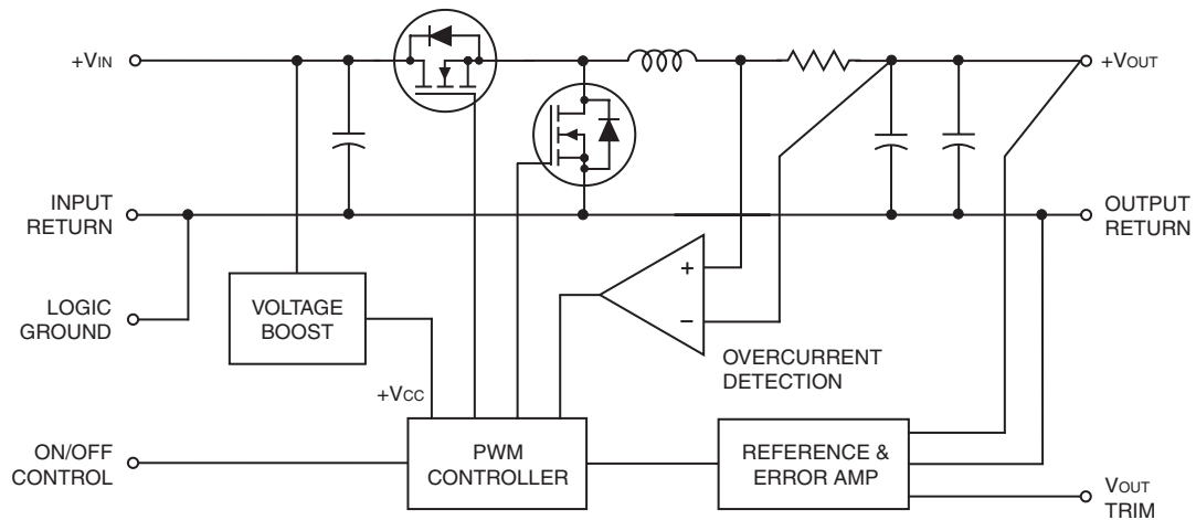
Figure 2. Simplified Schematic
