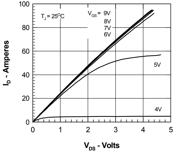
Fig. 1. Output Characteristics
