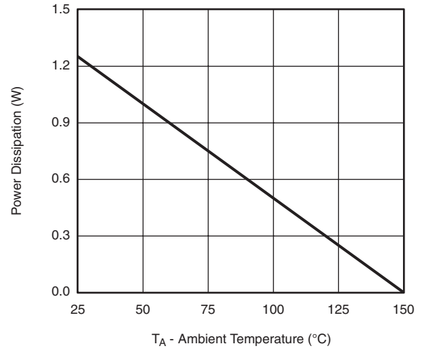
Power Derating
