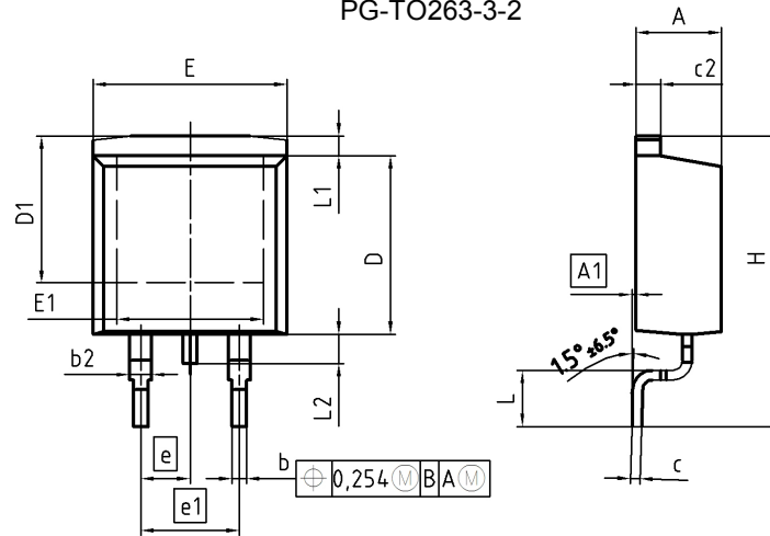
PG-TO263-3-2
