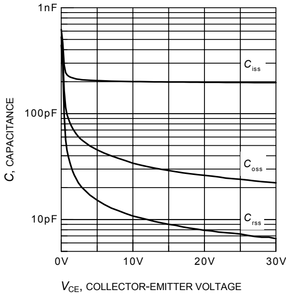
V_{CE} , COLLECTOR-EMITTER VOLTAGE Figure 19. Typical capacitance as a function of collector-emitter voltage ( V_{GE} = 0V, f = 1MHz )
