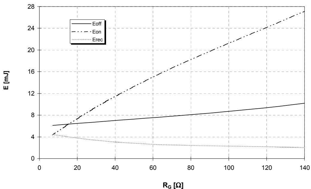
Schaltverluste (typisch) E_{on} = f(R_G) , E_{off} = f(R_G) , E_{rec} = f(R_G) Switching losses (typical) V_{GE} = \pm 15V , I_c = 50A , V_{CE} = 600V , T_{vj} = 125^\circ C
