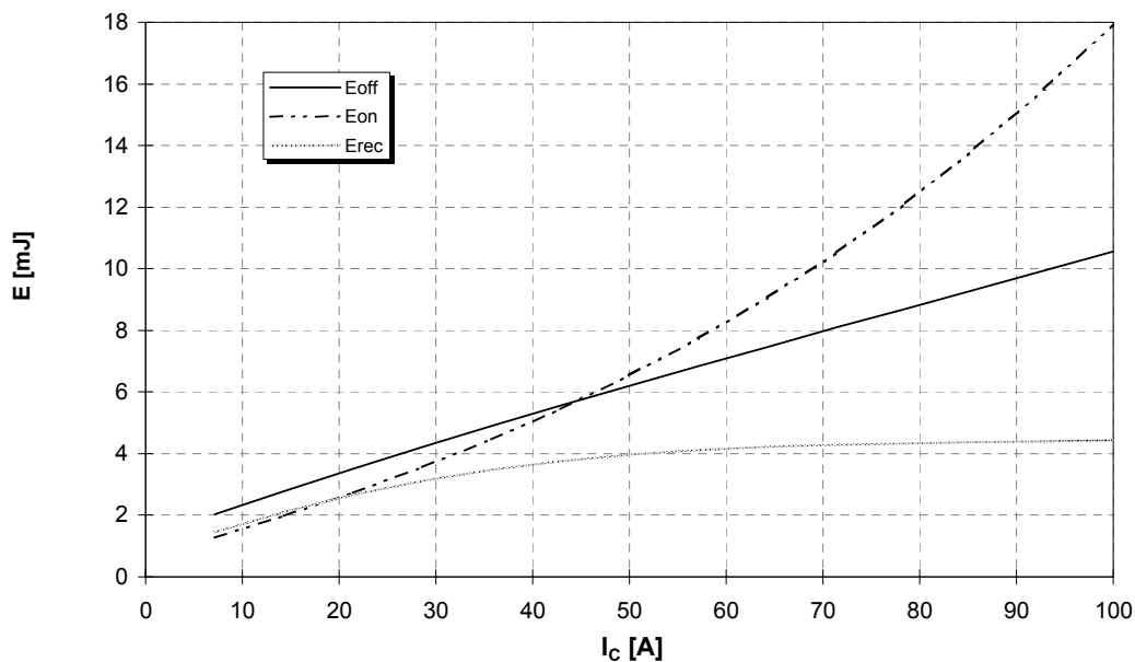
Schaltverluste (typisch) E_{on} = f(I_c) , E_{off} = f(I_c) , E_{rec} = f(I_c) Switching losses (typical) V_{GE} = \pm 15V , R_G = 15 \Omega , V_{CE} = 600V , T_{vj} = 125^\circ C
