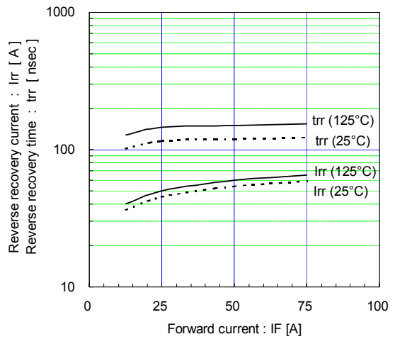
[ Inverter ] Reverse recovery characteristics (typ.) V_{cc}=600V, V_{GE}=\pm 15V, R_g=22\Omega
