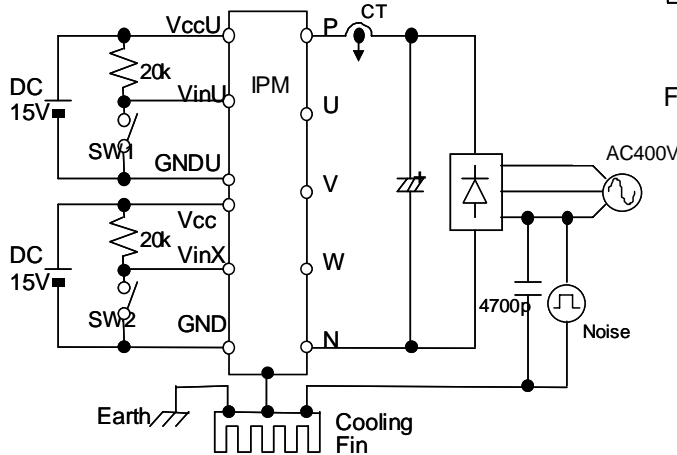
Figure 5. Noise Test Circuit
