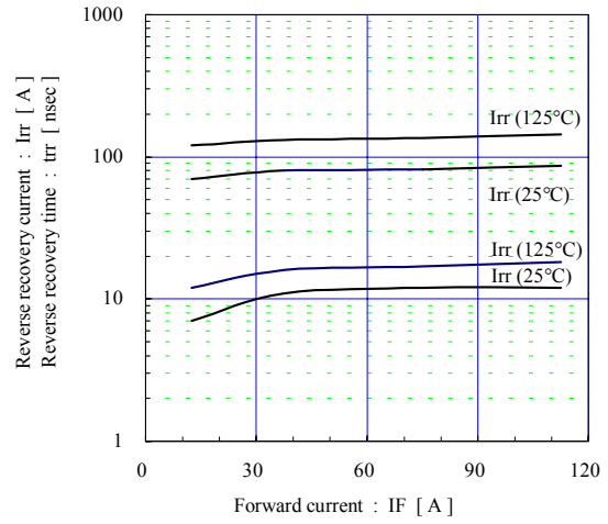
Reverse recovery characteristics (typ.) Vcc=300V, VGE=±15V, Rg=47Ω
