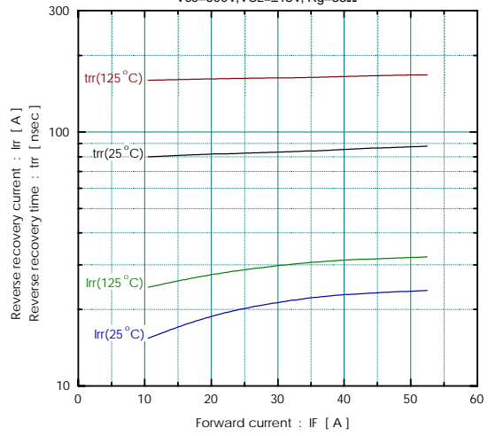
Reverse recovery characteristics (typ.) Vcc=600V, VGE=±15V, Rg=33Ω
