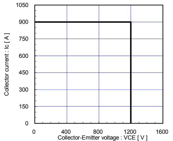
Reverse bias safe operating area (max.) +V_{GE}=15V, -V_{GE} \le 15V, R_G \ge 1.1\Omega, T_J \le 125^\circ C Stray inductance \le 100nH
