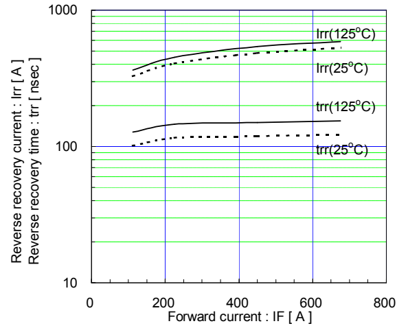
Reverse recovery characteristics (typ.) V_{CC}=600\text{V} , V_{GE}=\pm 15\text{V} , R_G=1.1\Omega
