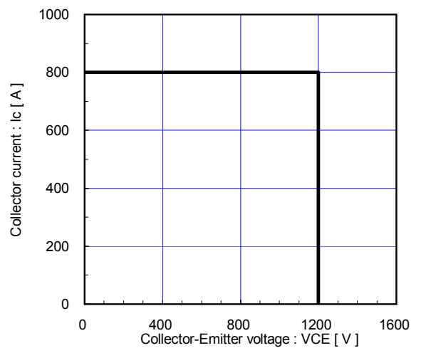
Reverse bias safe operating area (max.) +V_{GE}=15V, -V_{GE} \le 15V, R_G \ge 1.5\Omega, T_J \le 125^\circ C
