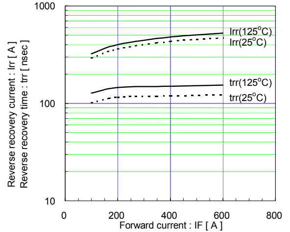
Reverse recovery characteristics (typ.) Vcc=600V, VGE=±15V, RG=1.5Ω
