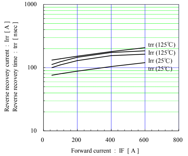
Reverse recovery characteristics (typ.) Vce=300V, VGE=±15V, Rg=6.8Ω
