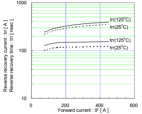
Reverse recovery characteristics (typ.) Vcc=600V, VGE=±15V, RG=2.0Ω
