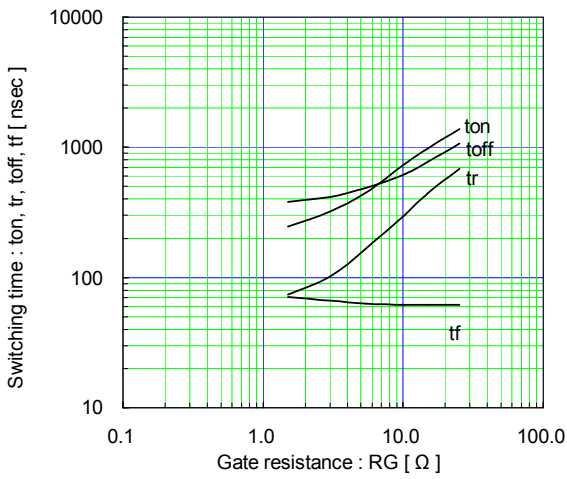
Switching time vs. Gate resistance (typ.) V_{CC}=600V, I_c=225A, V_{GE}=\pm 15V, T_J=25^\circ C
