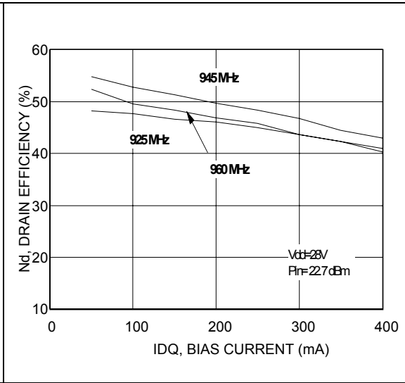
Figure 20. Drain efficiency vs bias current
