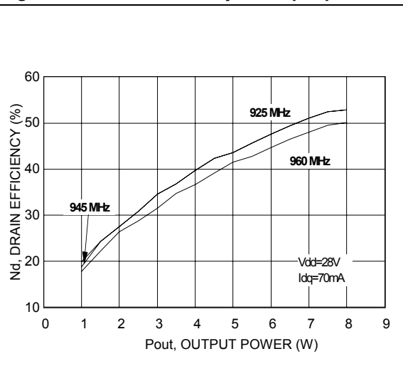
Figure 9. Drain efficiency vs output power
