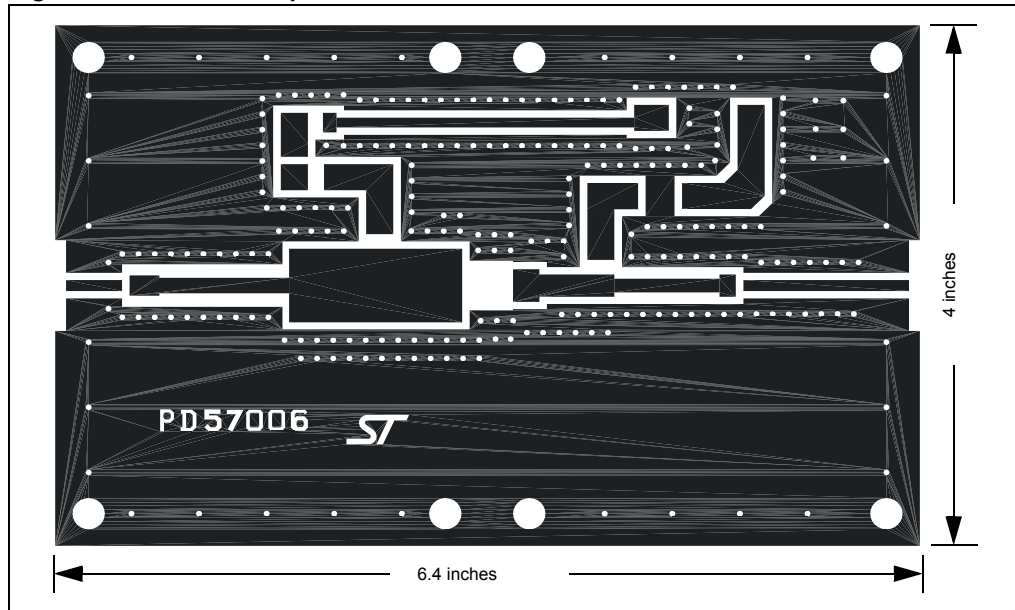
Figure 26. Test circuit
