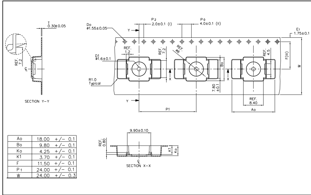
Figure 30. Reel information
