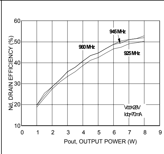
Figure 18. Drain efficiency vs output power
