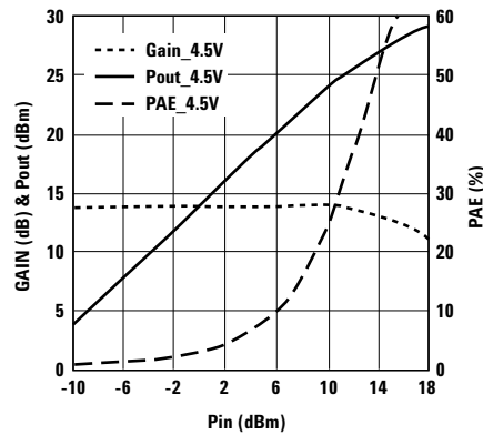
Figure 49. Small Signal Gain/Pout/PAE vs. P_{in} at V_{ds} 4.5V and Freq = 2.4\text{ GHz} .
