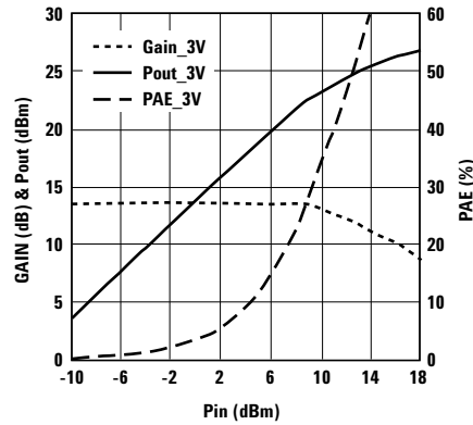
Figure 47. Small Signal Gain/Pout/PAE vs. P_{in} at V_{ds} 3V and Freq = 2.4\text{ GHz} .
