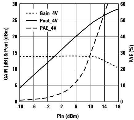
Figure 48. Small Signal Gain/Pout/PAE vs. P_{in} at V_{ds} 4V and Freq = 2.4\text{ GHz} .
