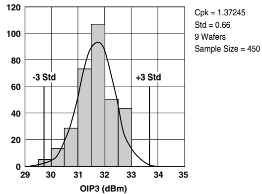
Figure 2. OIP3 @ 2 GHz, 4 V, 60 mA. LSL=29.0, Nominal=31.8, USL=35.0
