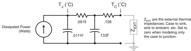
Figure 5b, TRANSIENT THERMAL IMPEDANCE MODEL
