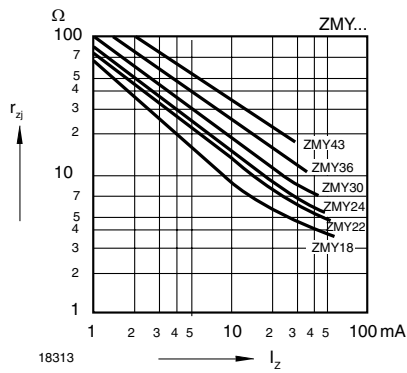
Figure 2. Dynamic Resistance vs. Zener Current
