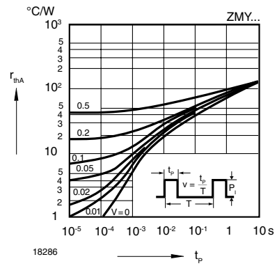
Figure 5. Pulse Thermal Resistance vs. Pulse Duration
