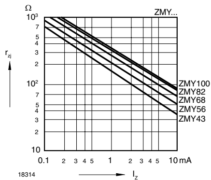
Figure 3. Dynamic Resistance vs. Zener Current
