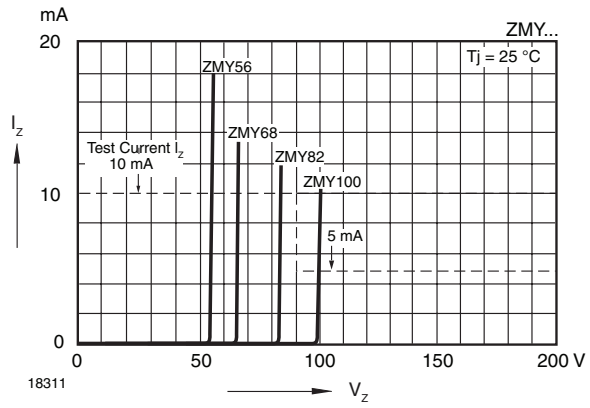
Figure 8. Breakdown Characteristics
