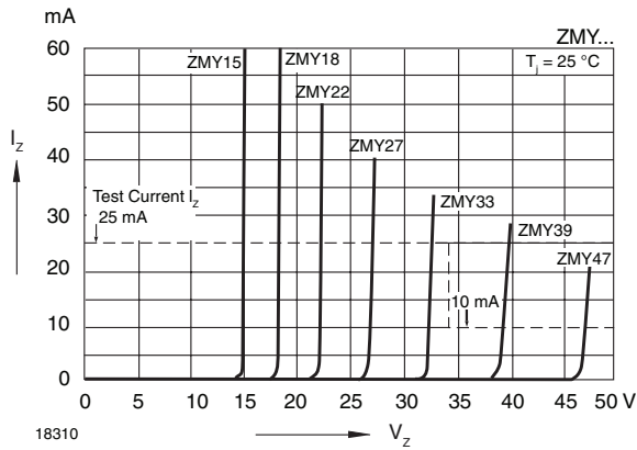
Figure 7. Breakdown Characteristics
