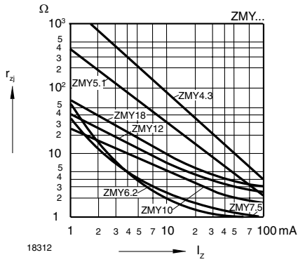
Figure 1. Dynamic Resistance vs. Zener Current
