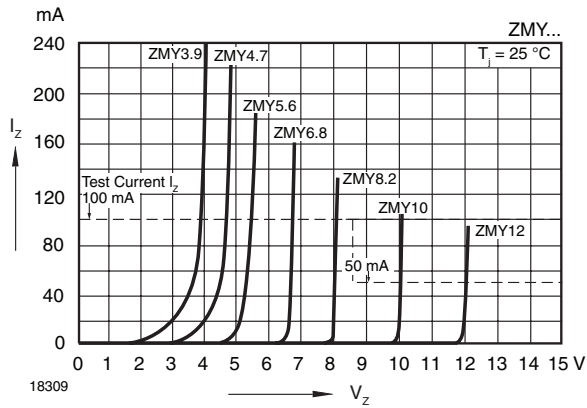
Figure 6. Breakdown Characteristics
