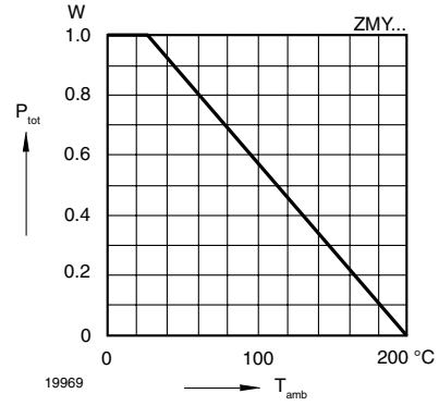
Figure 4. Admissible Power Dissipation vs. Ambient Temperature
