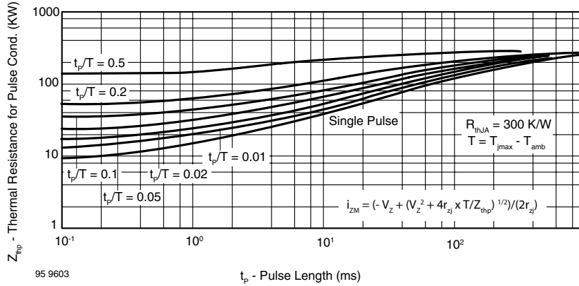
Figure 13. Thermal Response
