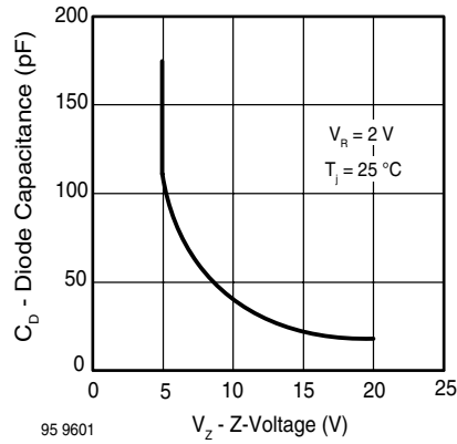
Figure 4. Diode Capacitance vs. Z-Voltage
