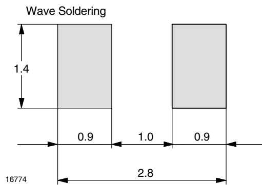
Figure 12. Recommended foot pads (in mm)
