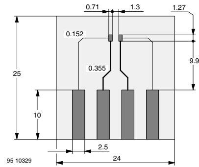
Figure 10. Board for R_{thJA} definition (in mm)
