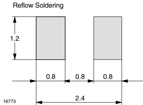
Figure 11. Recommended foot pads (in mm)
