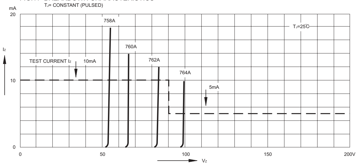
FIG.11- BREAKDOWN CHARACTERISTICS
