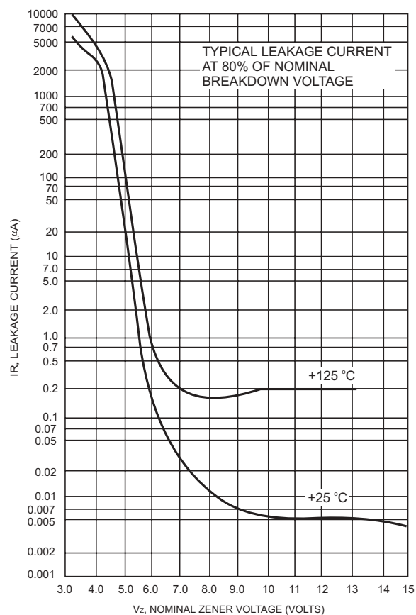
FIG.5- TYPICAL LEAKAGE CURRENT
