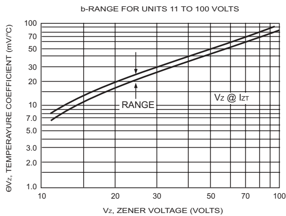
FIG.7- TEMPERATURE COEFFICIENTS
