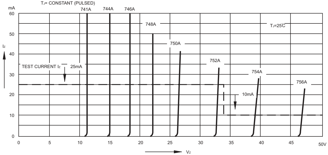
FIG.11- BREAKDOWN CHARACTERISTICS
