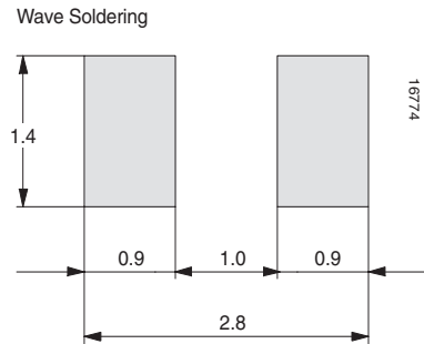
Figure 11. Recommended foot pads (in mm)
