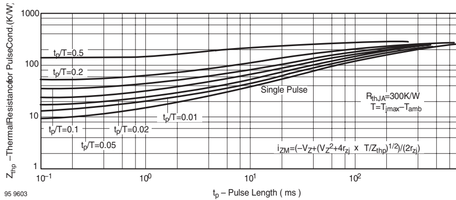
Figure 13. Thermal Response
