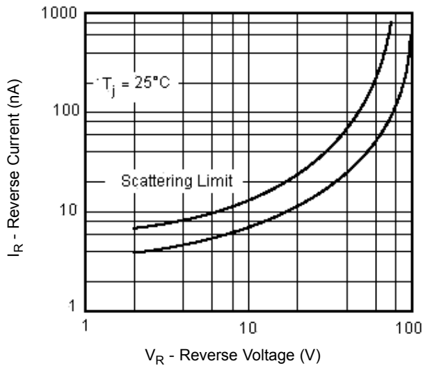
Reverse Current vs. Reverse Voltage
