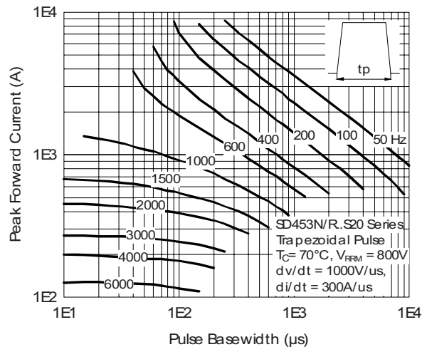
Fig. 27 - Frequency Characteristics
