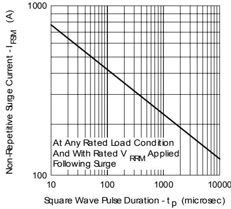
Fig. 7 - Max. Non-Repetitive Surge Current
