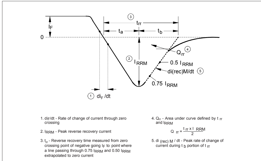
Fig. 12 - Reverse Recovery Waveform and Definitions
