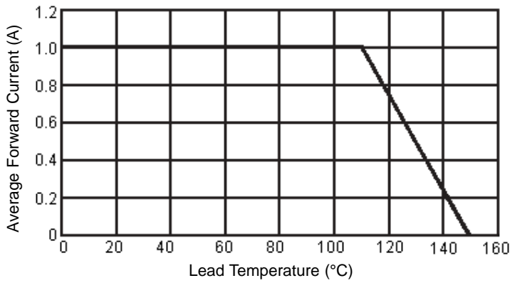
Maximum Forward Current Derating Curve
