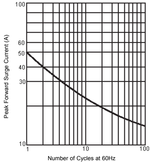
Maximum Non-Repetitive Forward Surge Current
