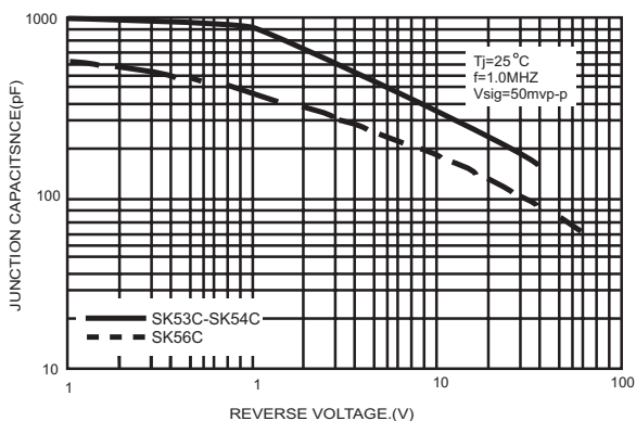
FIG.5-TYPICAL JUNCTION CAPACITANCE
