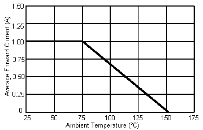
Figure 2 Maximum Forward Current Derating Curve
