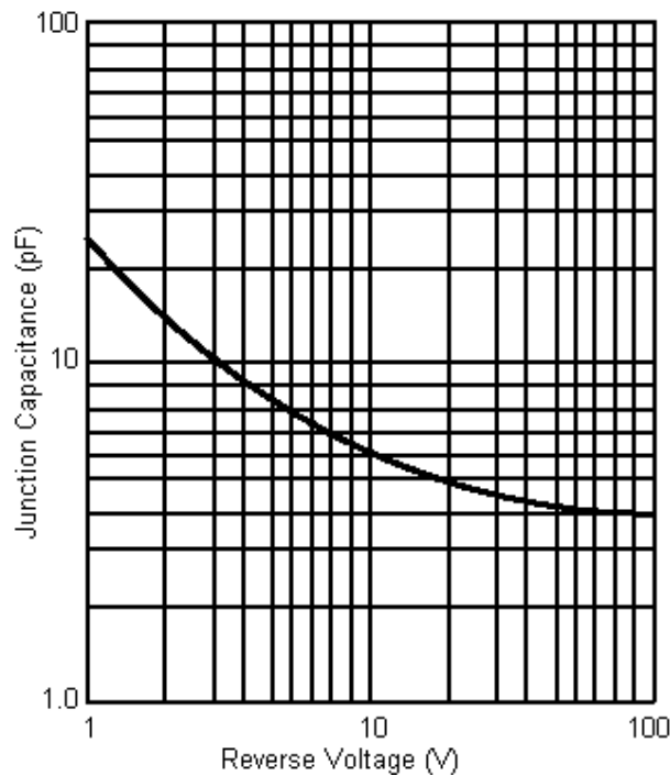
Figure 3 Typical Junction Capacitance
