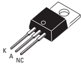
TO-220AB Isolated (CRNA25...L3)
