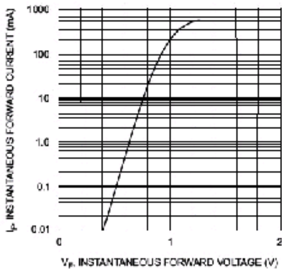
Fig. 1 Forward Characteristics
