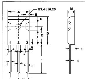
TO-247 (3P)
