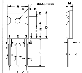
TO-247 (3P)
