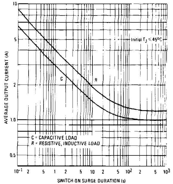
Fig. 4 – Maximum Switch-On Surge Current Vs. Surge Duration
