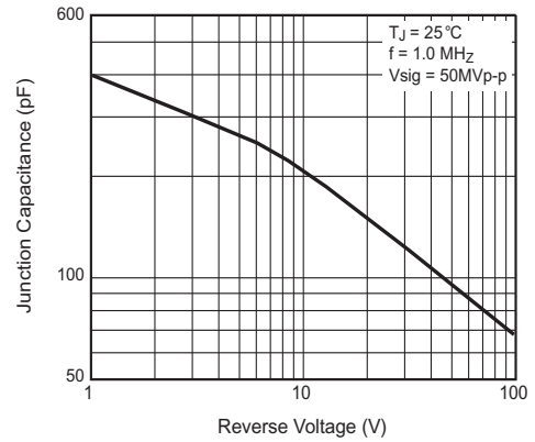
Figure 7. Typical Junction Capacitance Per Leg
