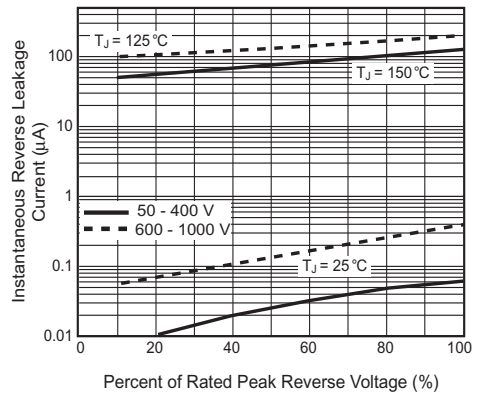
Figure 6. Typical Reverse Leakage Characteristics Per Leg
