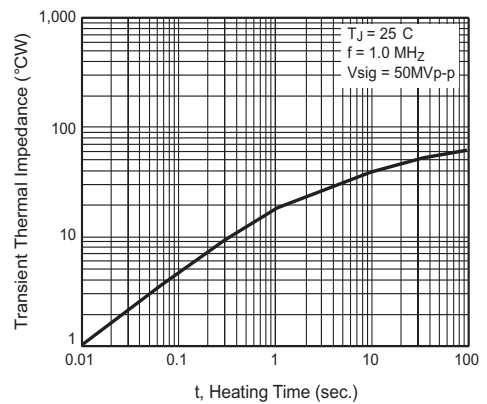
Figure 8. Typical Transient Thermal Impedance Per Leg
