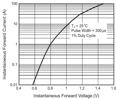
Figure 5. Typical Instantaneous Forward Characteristics Per Leg
