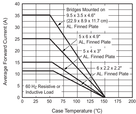
Figure 1. Maximum Output Rectified Current
