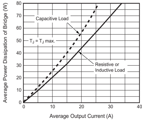
Figure 3. Maximum Power Dissipation
