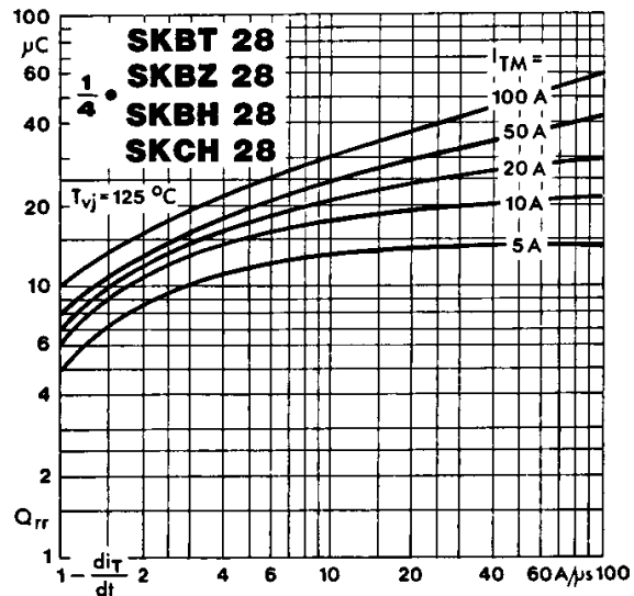
Fig. 8 Recovered charge vs. current decrease
