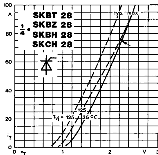
Fig. 10 On-state characteristics of a single thyristor
