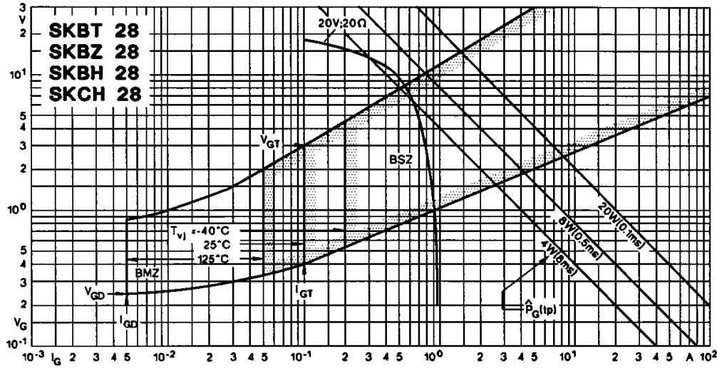
Fig. 11 Gate trigger characteristics
