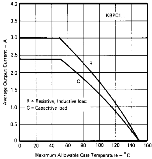
Fig. 1 – Case Temperature Ratings
