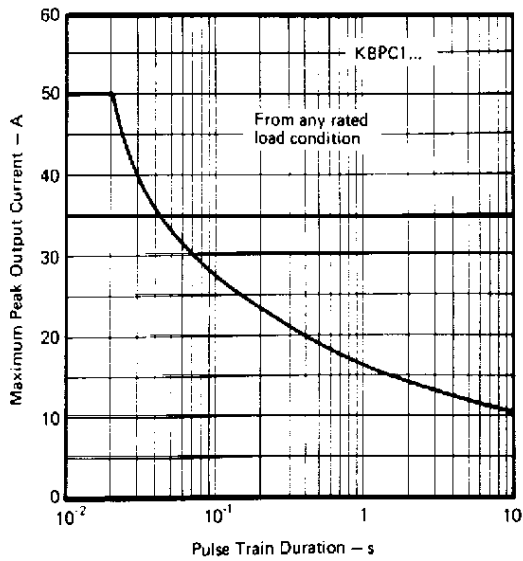
Fig. 3 – Non-Repetitive Surge Ratings
