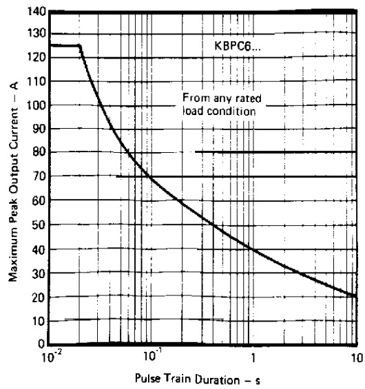
Fig. 4 – Non-Repetitive Surge Ratings
