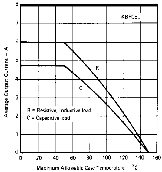
Fig. 2 – Case Temperature Ratings
