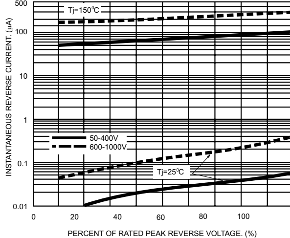
FIG.4- TYPICAL REVERSE CHARACTERISTICS PER BRIDGE ELEMENT
