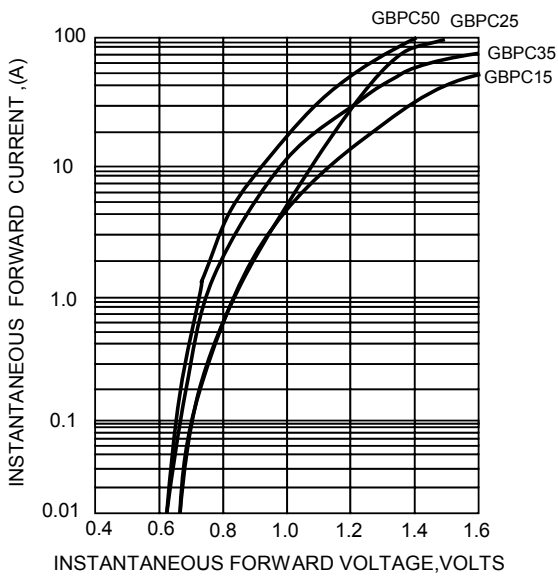
FIG.3-TYPICAL FORWARD CHARACTERISTICS
