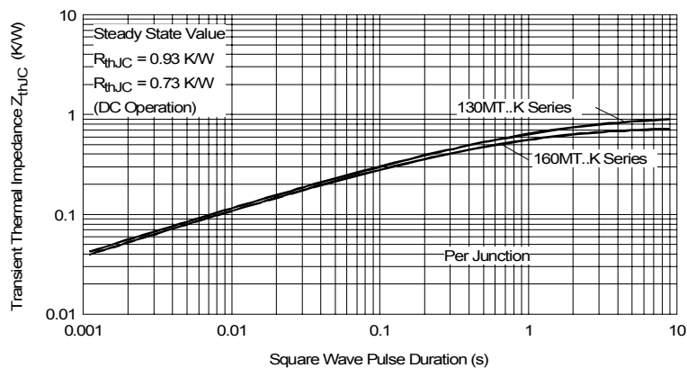
Fig. 11 - Thermal Impedance Z_{thJC} Characteristic
