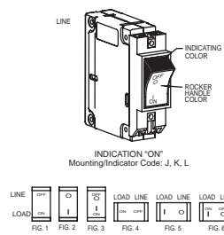
MARKING DETAIL "B" (SEE TABLE)
