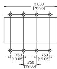
Panel Mounting Detail Tolerance ±.005 [.13] unless noted.
