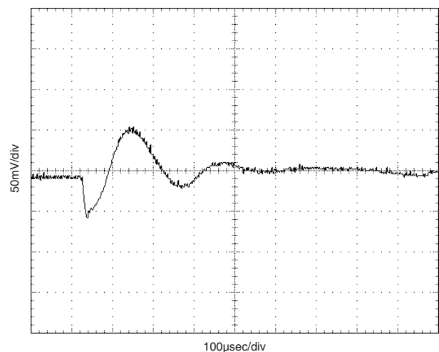
Dynamic Load Response (VIN = 3.3V, VOUT = 2.5V, 0% to 100% Load Step, COUT = 5000μF OSCON)
