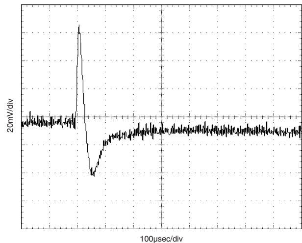
Dynamic Load Response (VIN = 3.3V, 100% to 50% Load Step, COUT = 220μF)
