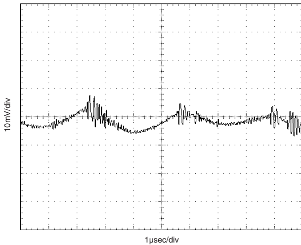
Output Ripple/Noise (VIN = 3.3V, VOUT = 2.5V, Full Load, COUT = 220μF)
