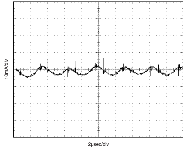
Input Reflected Ripple Current (V IN = 5V, V OUT = 3.3V/10A, Input Filter = 220μF/12μH/33μF, C OUT = NA)
